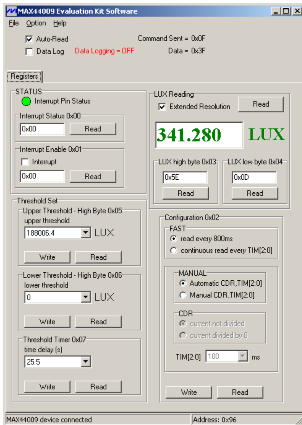
Figure 1. MAX44009 EV Kit Software Main Window
